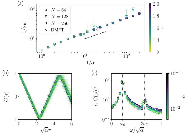
Figure 6.8: Evolution of the oscillation frequency \omega_0 with the memory loss rate \alpha for \beta \rightarrow \infty , \varepsilon > 2 - \varepsilon_c averaged over 96 samples of disorder and initial conditions, errorbars showing 95% confidence interval. (a) Log-log plot of \omega_0 as a function of \alpha , dashed line corresponding to \omega_0 \sim \sqrt{\alpha} . (b) Two-point autocorrelation for \varepsilon = 1.8 , N = 256 as a function of the rescaled time lag for different values of \alpha . (c) Power spectrum of the autocorrelation for the same parameters, displaying secondary peaks at odd multiples of this fundamental frequency, as expected from the triangular aspect of C(\tau) .
