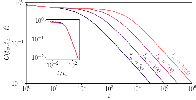
Figure 2.2: Two-point correlation function in the spherical SK model at T = 0.3 for different system ages, taken from [123]. Inset: same quantity represented as a function of the time rescaled by the age, t/t_w , showing a clear collapse in the aging regime.
