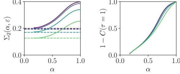
Figure 6.2: (a) L = 2 cycle complexity from the numerical resolution of the saddle point equations for \varepsilon = \{0, 0.2, 0.4, 0.6\} from dark purple to light green, dashed lines indicating the fixed point complexity associated to each parameter. (b) Overlap between successive steps C(\tau = 1) = -i\hat{R}(t, t + 1) at the L = 2 saddle, showing the nontrivial coalescence of the cycle and fixed point saddle point solutions as \alpha is decreased. The numerical resolution appears to breakdown when we get close to \alpha = 0 .
