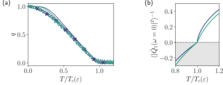
Figure 6.10: (a) Order parameter q = C(t, t) averaged in time in the (quasi) stationary regime vs. rescaled temperature for \varepsilon = \{0.1, 0.4\} (dark and light shades respectively). Circular and diamond markers correspond direct, finite size simulations at N = 256 for \alpha = 0.01 and \alpha = 0.1 respectively, whereas crosses represent the (dynamical) numerical solution to the complete set of N \rightarrow \infty DMFT equations for \alpha = 0.1 . Continuous lines show the solutions to the static DMFT fixed point equations (Eq. (6.23)-(6.25)). (b) Spectral density of a small perturbation Q_1 to the fixed point solution of the DMFT close to the critical temperature. As the quantity is necessarily positive for a valid solution, the grey region corresponds to instability.
